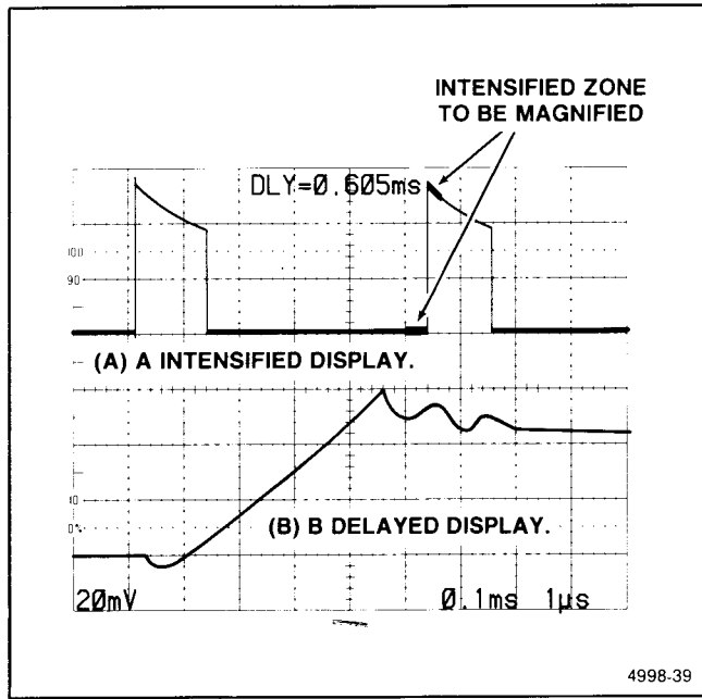
Figure 6-26. Delayed-sweep magnification.
