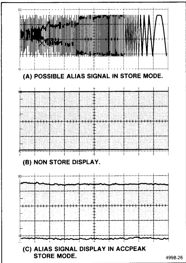
Figure 6-13. Anti-aliasing.
