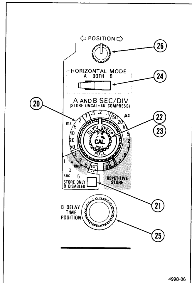
Figure 3-3. Horizontal controls.
