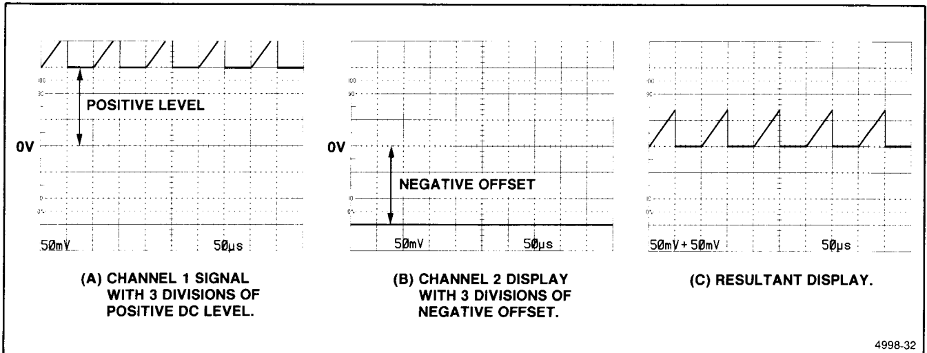
Figure 6-19. Algebraic addition.
