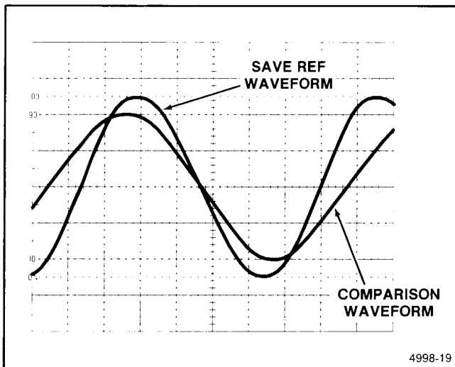
Figure 6-6. Waveform comparison.
