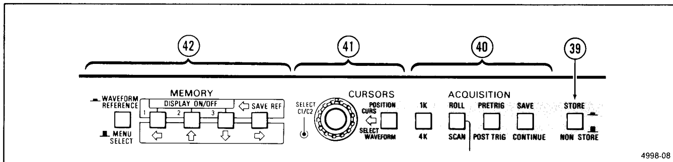
Figure 3-5. Storage controls.
