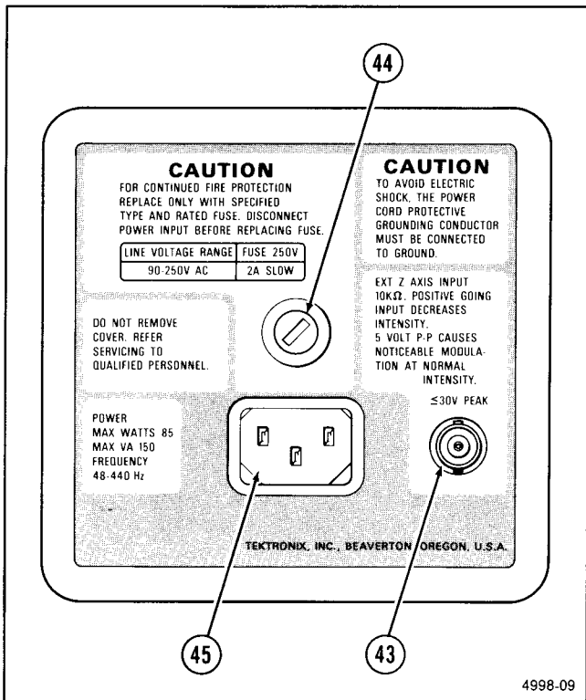
Figure 3-6. Rear panel.
