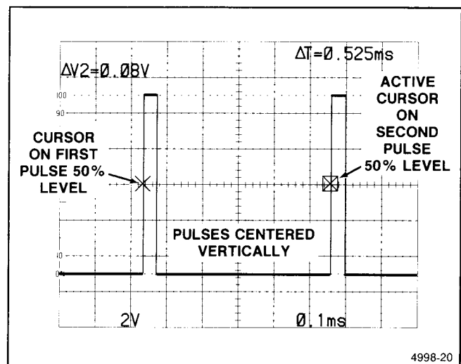
Figure 6-7. Time difference between repetitive pulses.
