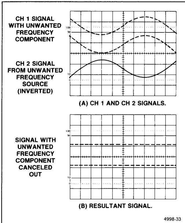
Figure 6-20. Common-mode rejection.
