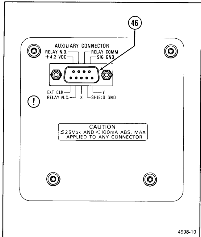
Figure 3-7. Side panel.
