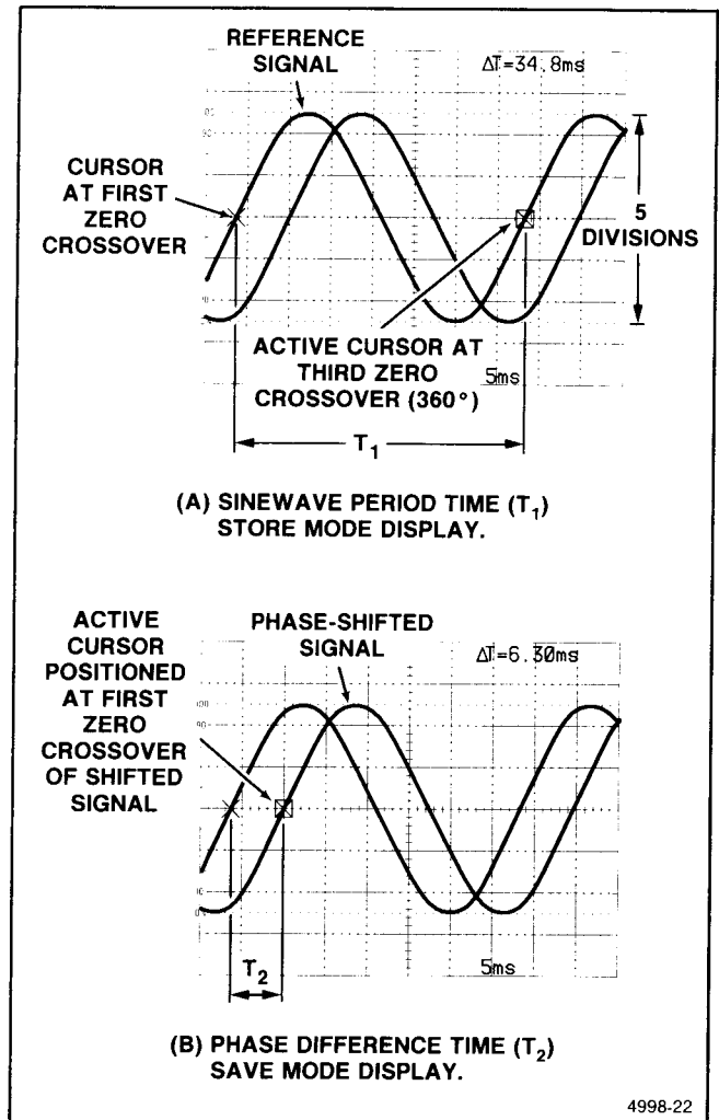
Figure 6-9. Phase difference between sinusoidal signals.
